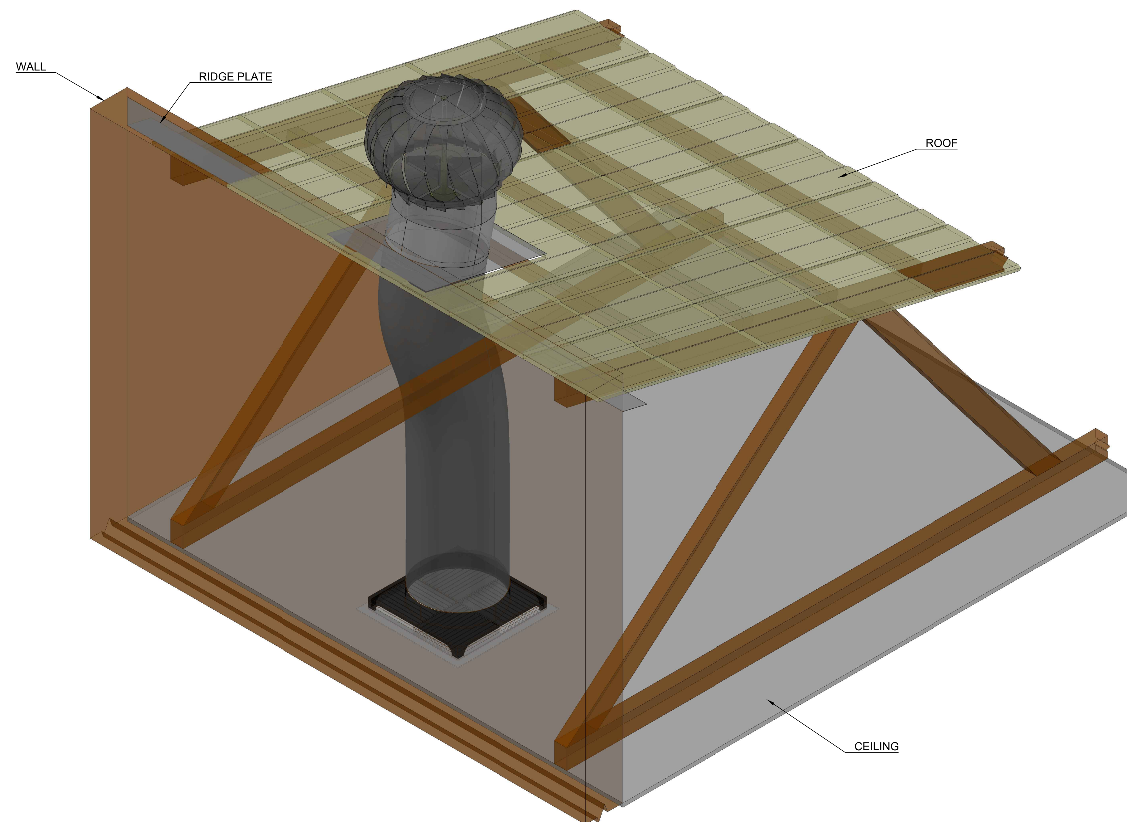
FLEXIBLE DUCTING COLLAR TO BE PRE ORDERED AND FITTED IN FACTORY
